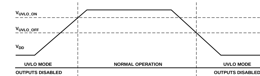
Figure 5. UVLO Function
