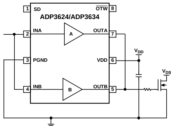
Figure 25. Parallel Operation
