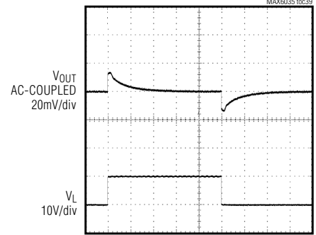
MAX6035 LOAD TRANSIENT ( V_{OUT} = 5V )
