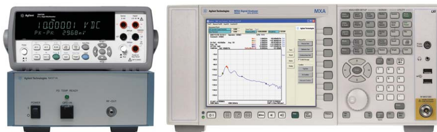
Figure 1. N4371A RIN Measurement System
