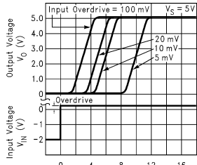
Response Time for Various Input Overdrives -t_{PLH}
