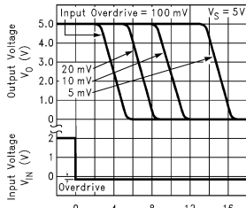
Response Time for Various Input Overdrives -t_{PHL}
