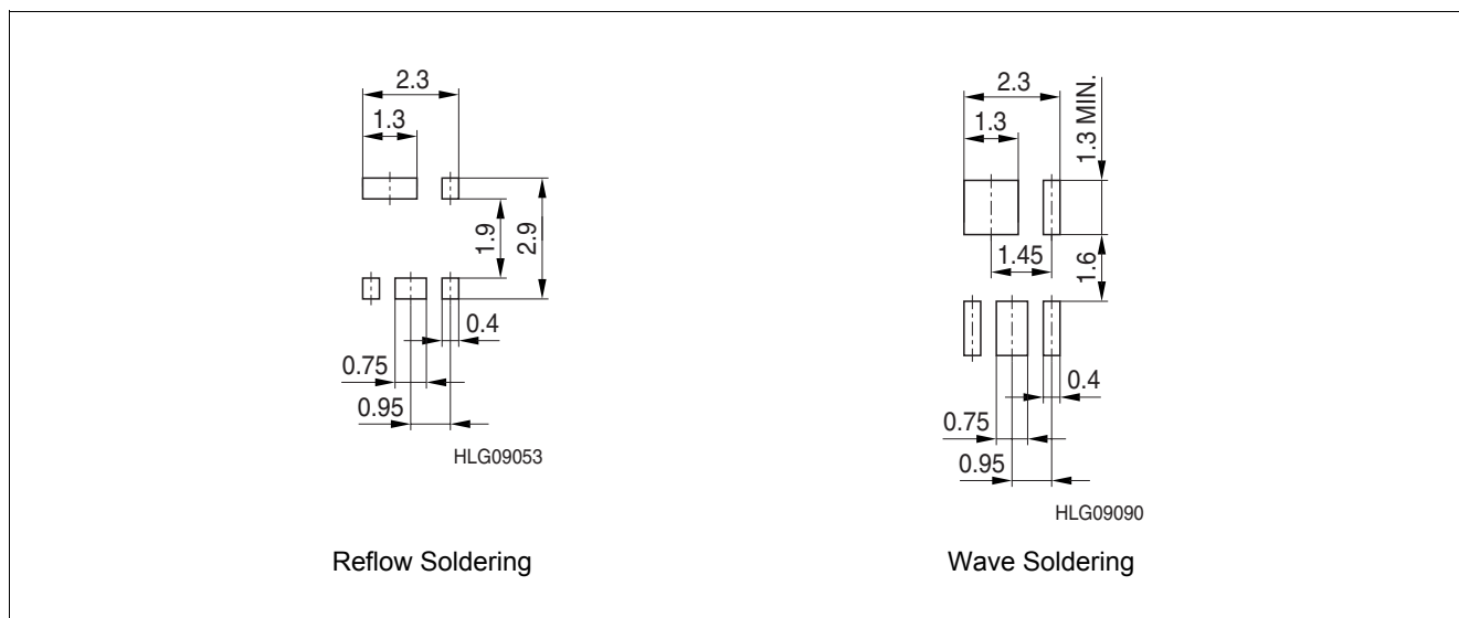
Figure 4 Footprint PG-SCT595-5
