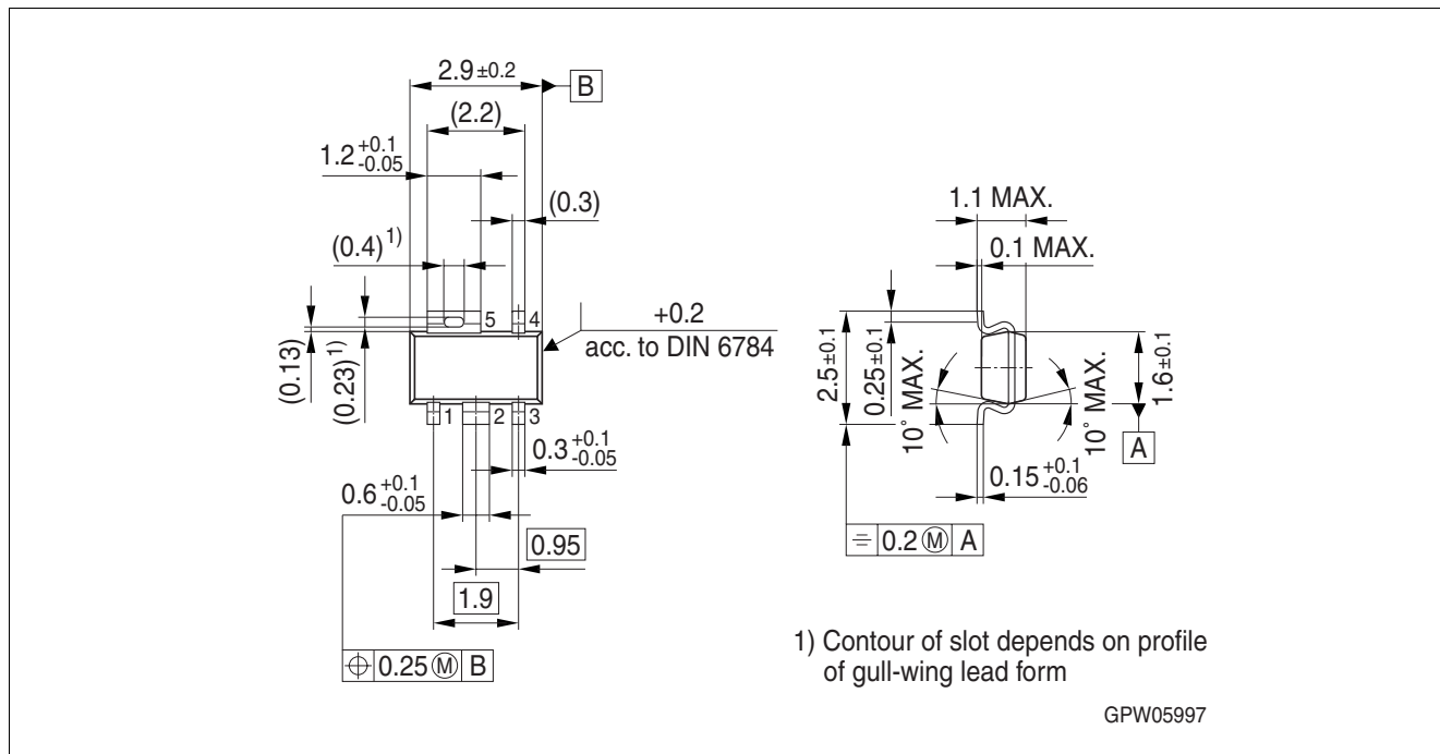
Figure 3 Outline PG-SCT595-5
