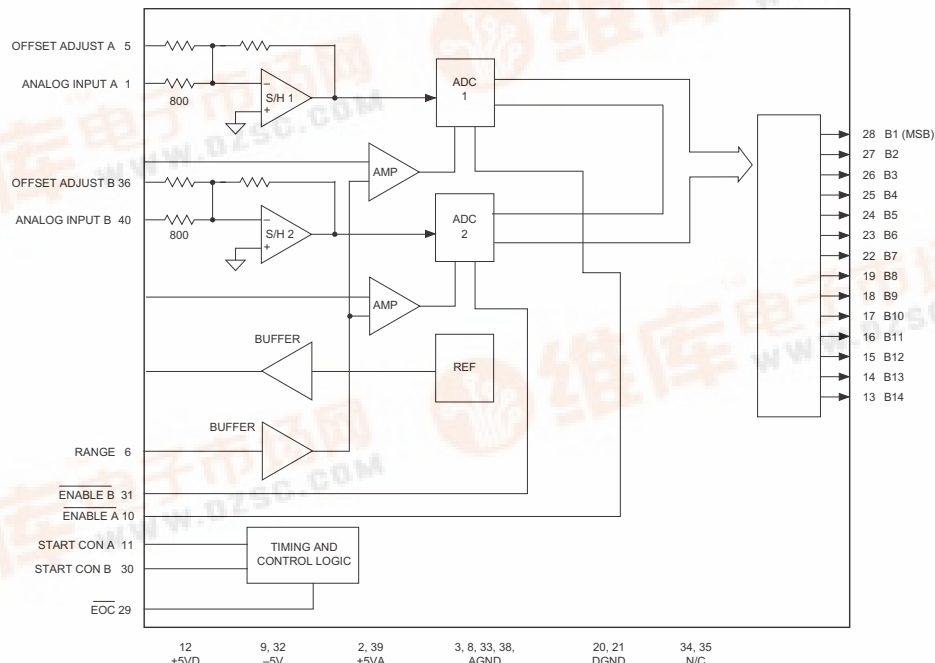
Figure 1. ADSD-1402 Functional Block Diagram
