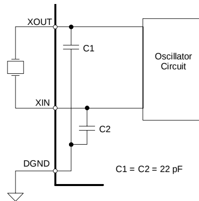
Figure 6. Oscillator Connections
