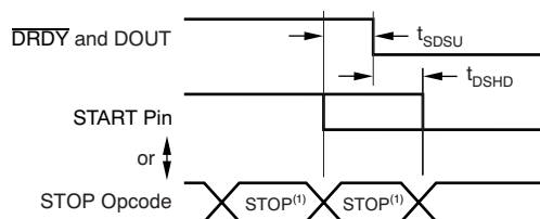
Figure 37. START to DRDY Timing
