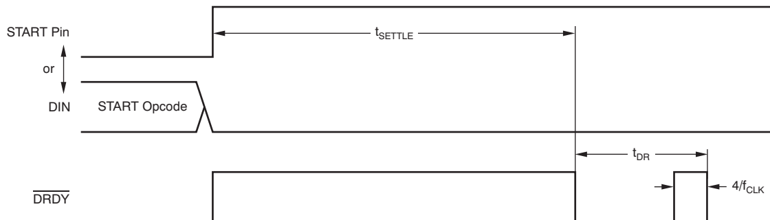
Figure 35. Settling Time
