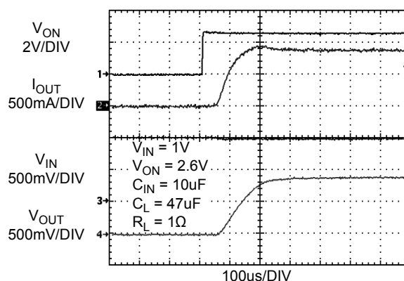
Figure 14. FPF1017 / 18 Turn On response
