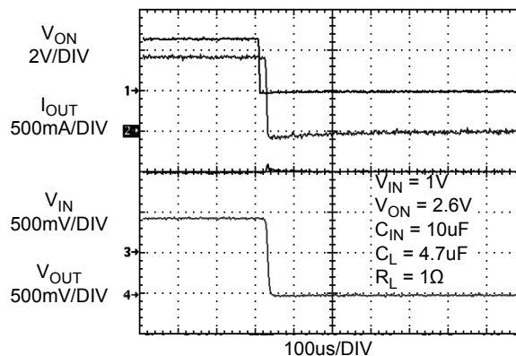
Figure 18. FPF1016 / 18 Turn OFF response
