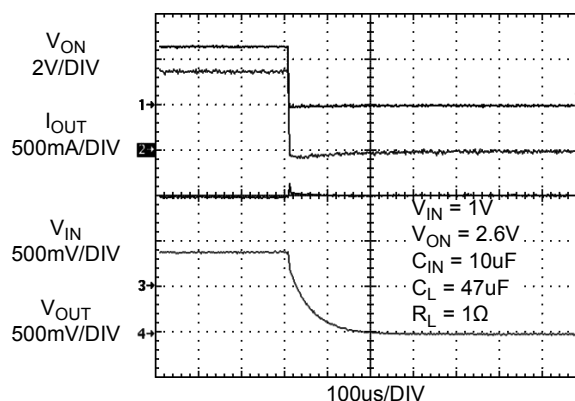
Figure 16. FPF1015 / 17 Turn OFF response
