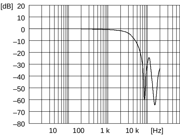
Figure 10.1 LPF Frequency Characteristics ( f_{SAM} = 8\text{ kHz} )
