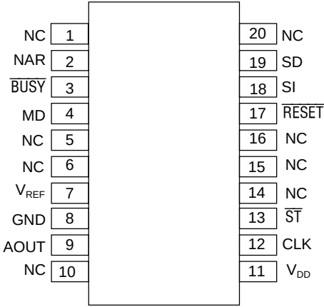
20-Pin Plastic SSOP
