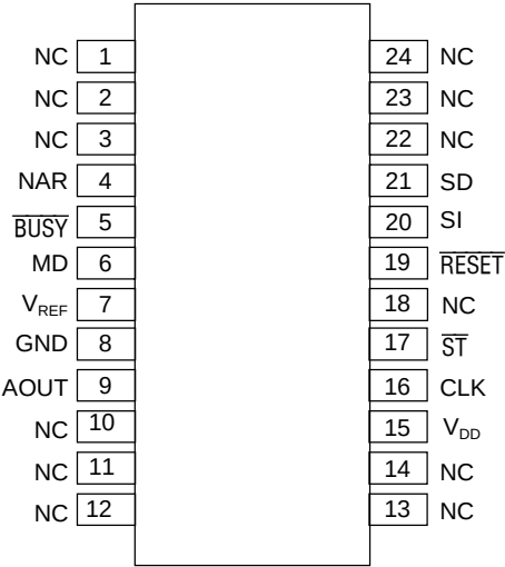
24-Pin Plastic SOP
