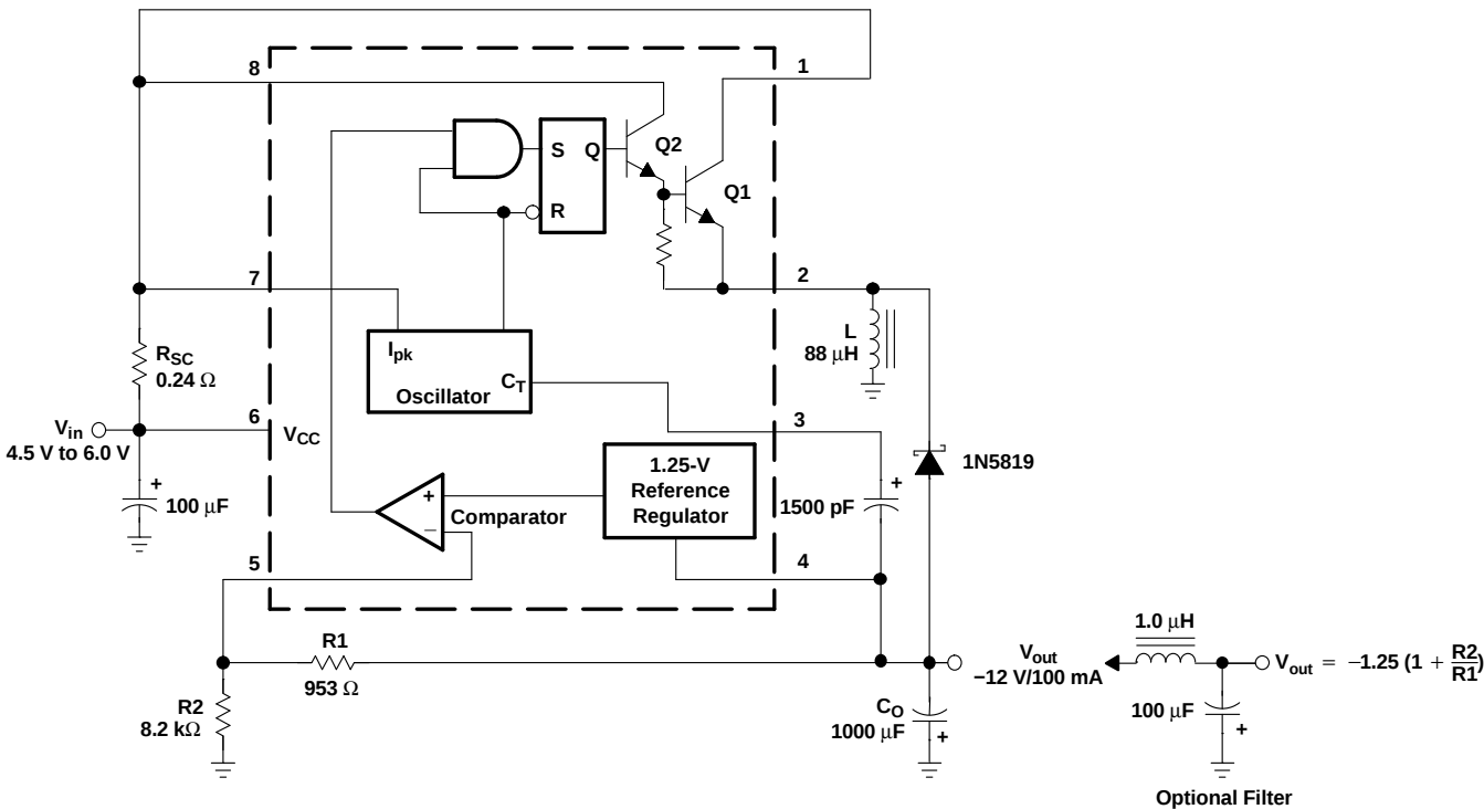
Figure 10. Voltage-Inverting Converter
