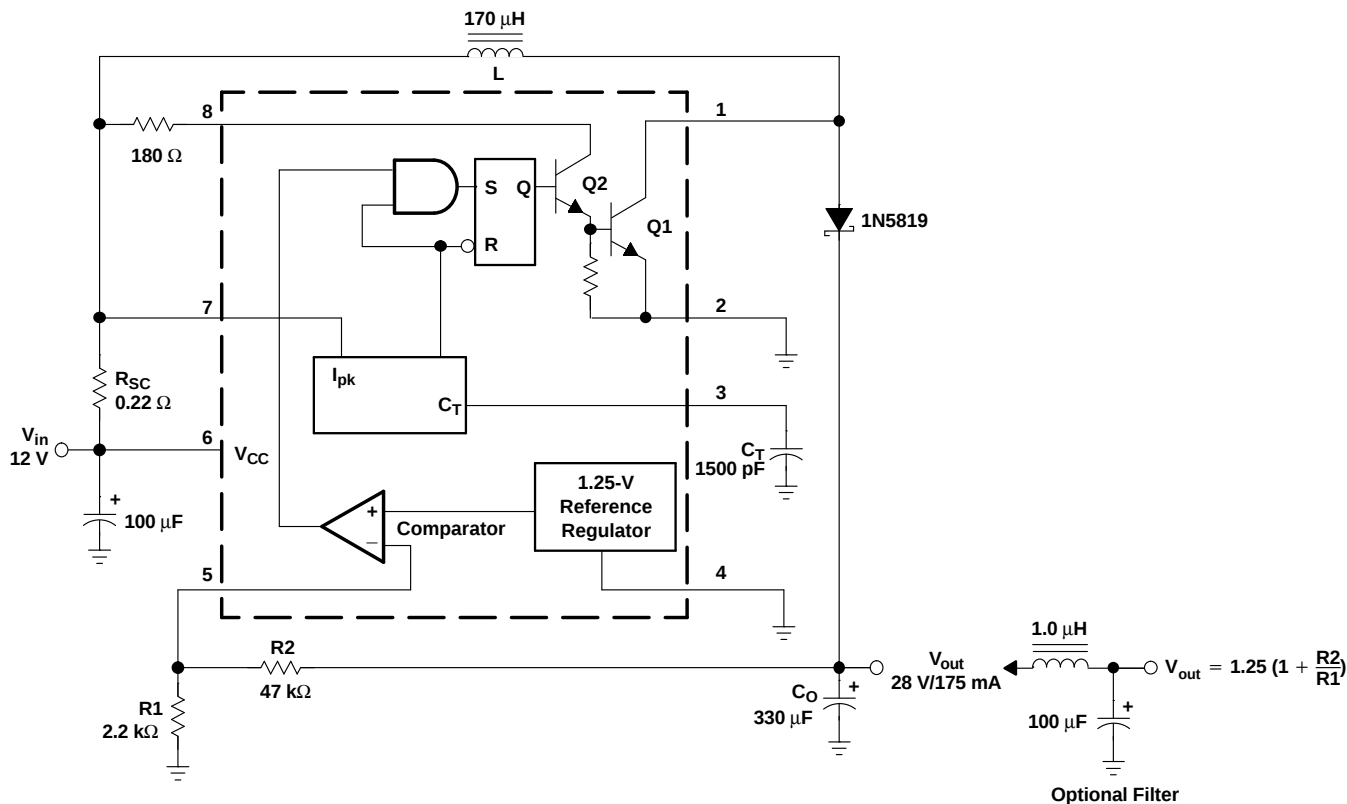
Figure 6. Step-Up Converter
