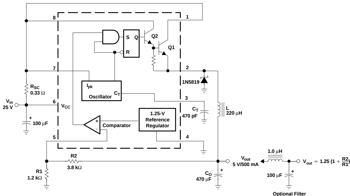
Figure 8. Step-Down Converter
