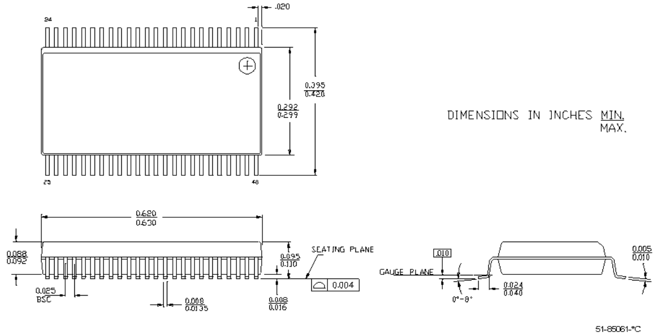
Figure 19. 48-Pin SSOP (51-85061)
