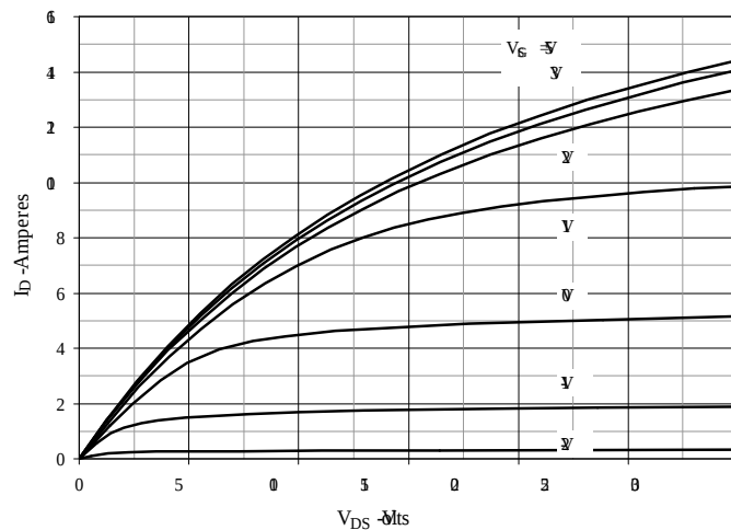
Fig2. Extended I_{DS} Characteristics @ T_J = 25^\circ\text{C}
