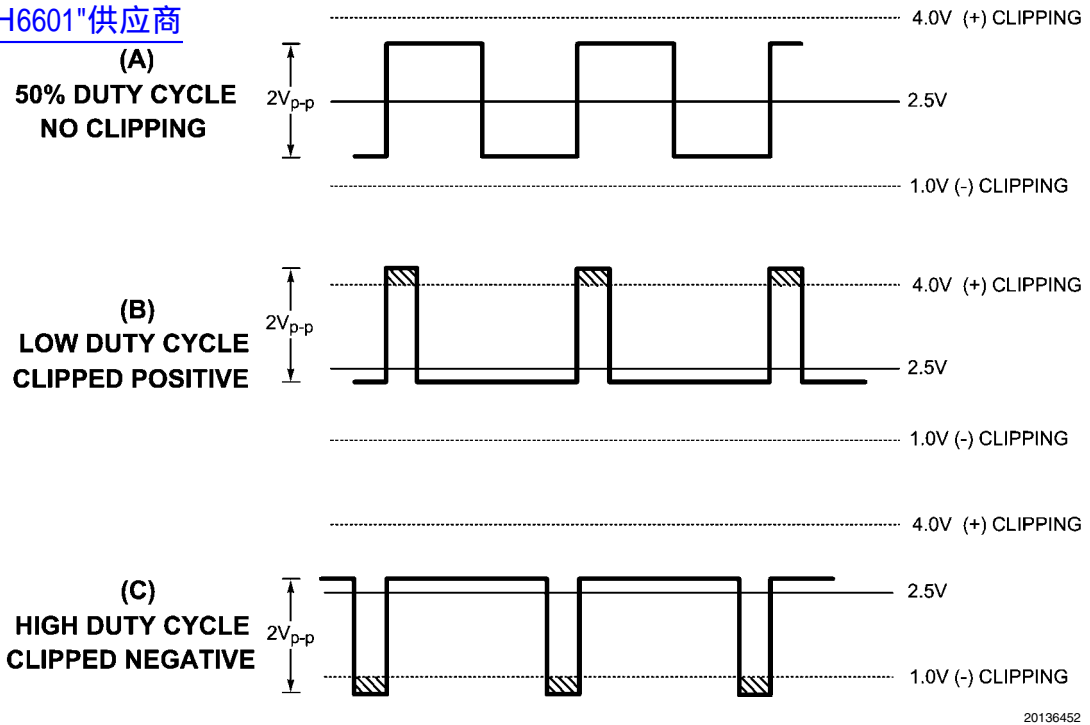
FIGURE 11. Headroom Considerations with AC Coupled Amplifiers
