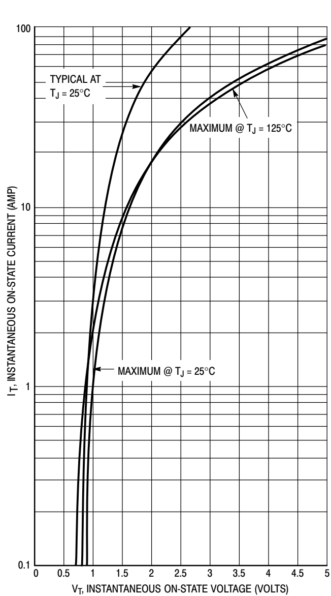
Figure 3. On-State Characteristics
