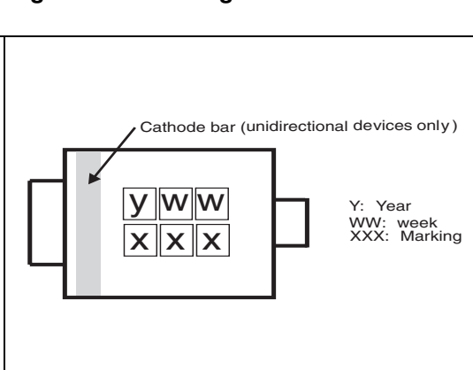
Figure 12. Marking information
