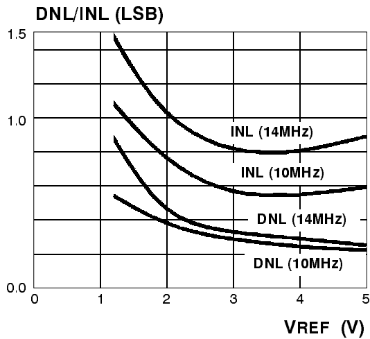
Accuracy (DNL/INL) vs. Reference Voltage ( V_{REF} ) vs. Sampling Rate ( F_S = 10, 14\text{ MHz} ) ( V_{IN\text{ }p-p} = V_{REF} )
