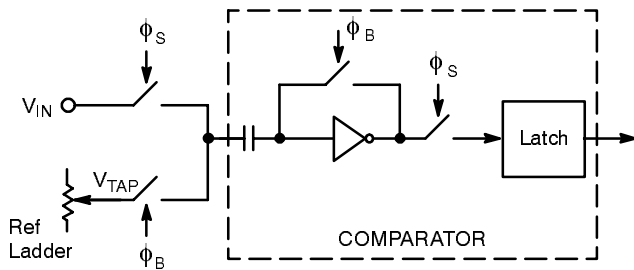
Figure 10. MP7690A Comparator
