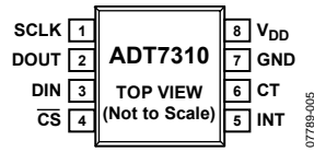
Figure 5. Pin Configuration
