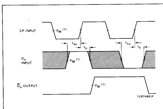
Fig. 8 Waveforms showing the data set-up and hold times for D_n input.
