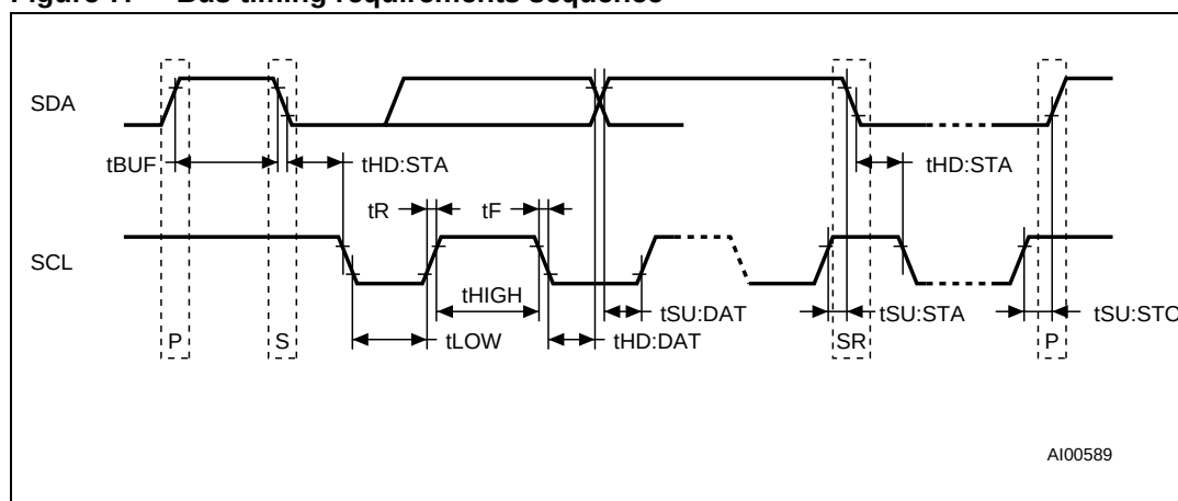
Figure 7. Bus timing requirements sequence
