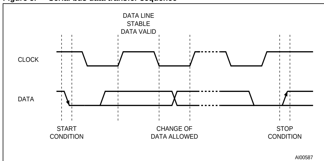
Figure 5. Serial bus data transfer sequence
