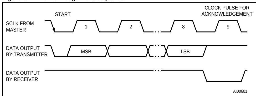
Figure 6. Acknowledgement sequence
