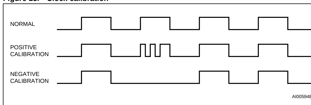
Figure 13. Clock calibration
