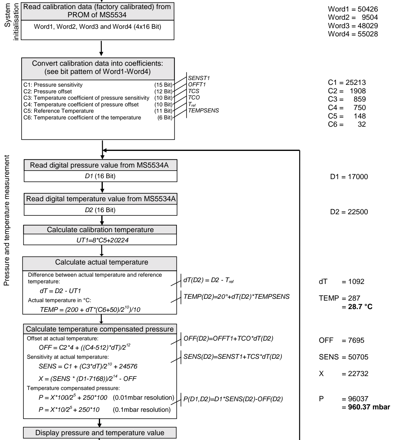
Fig. 3: Flow chart for pressure/temperature reading and software compensation.
