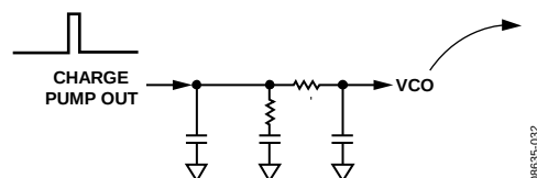
Figure 34. Typical Loop Filter Configuration
