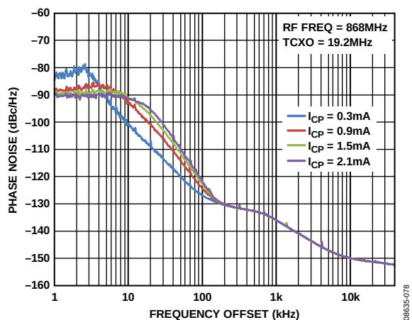
Figure 12. Phase Noise Response at 868 MHz, V_{DD} = 2.3V
