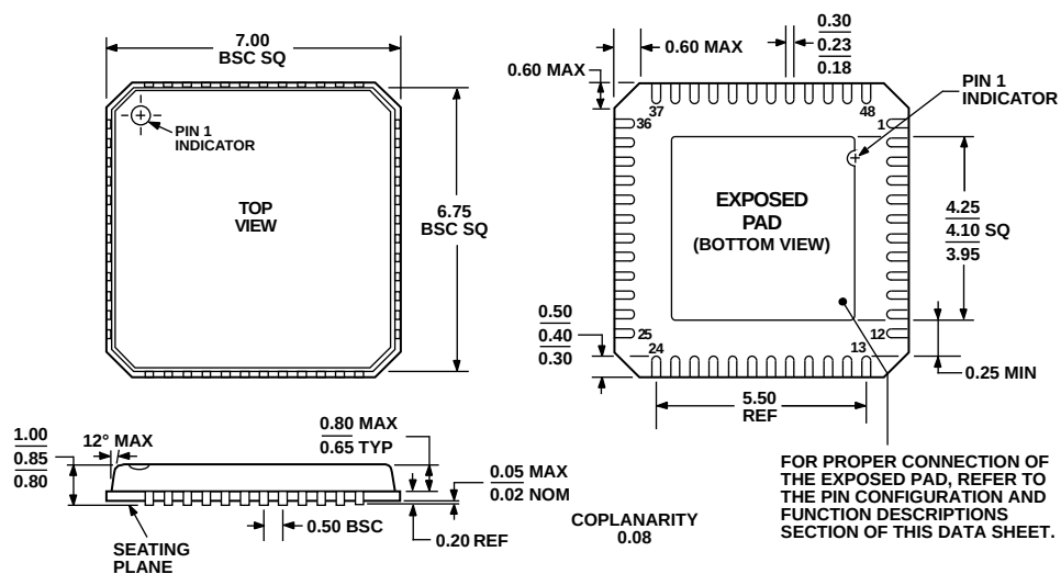
Figure 78. 48-Lead Lead Frame Chip Scale Package [LFCSP_VQ]
