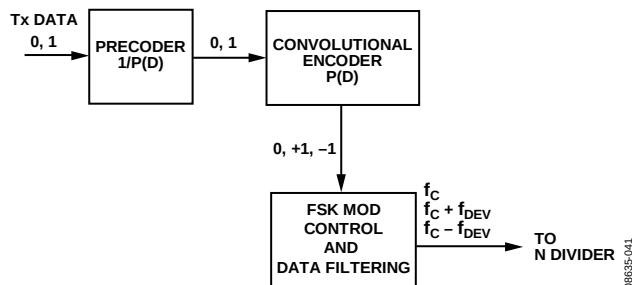
Figure 42. 3FSK Encoding
