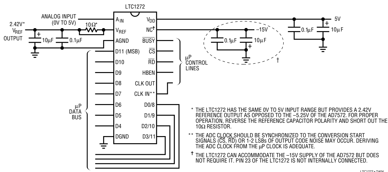
Figure 22. Plugging the LTC1272 into an AD7572 Socket
