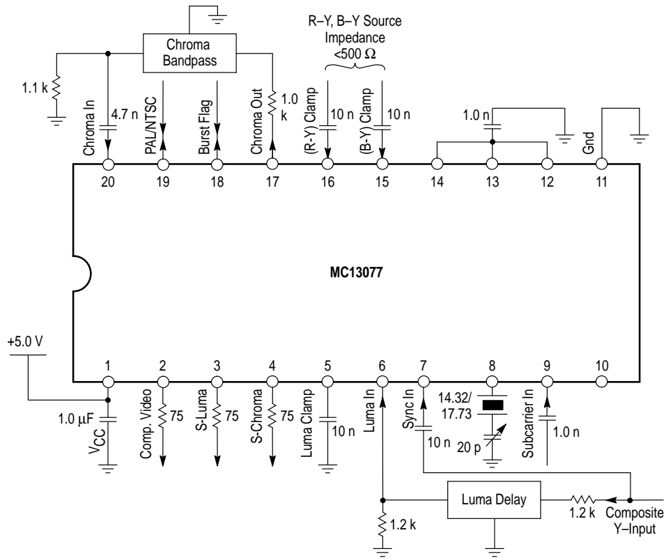
Figure 13. Encoder with Composite Luma and Color Difference Inputs 查询"MC13077"供应商 Using the Sync Separator and Having Phase-Locked Subcarrier
