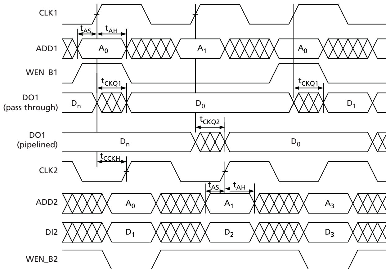
Figure 2-38 • Write Access after Read onto Same Address
