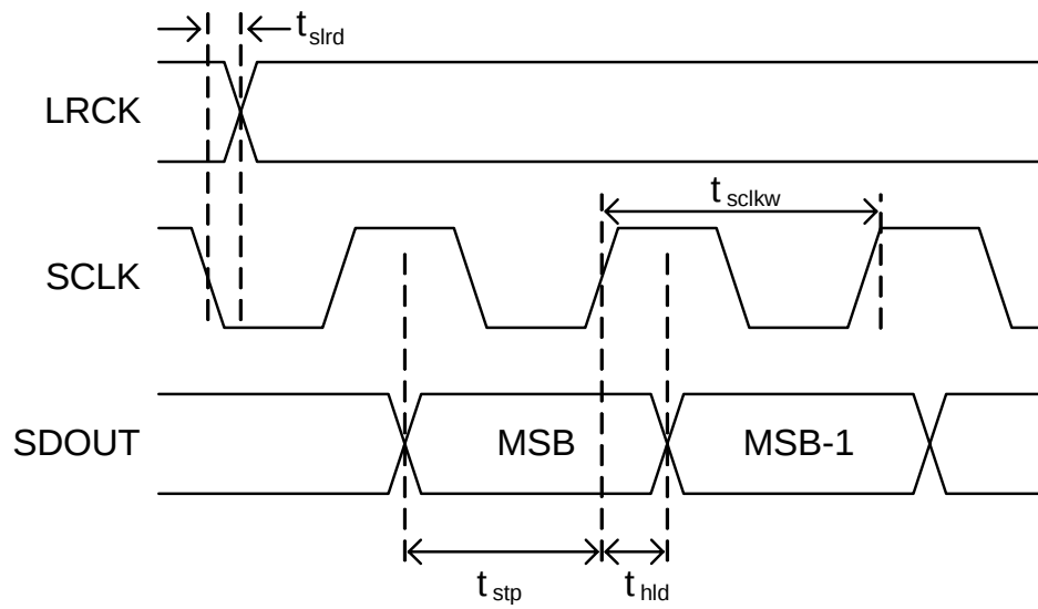
Figure 1. CS5343 I²S Serial Audio Interface
