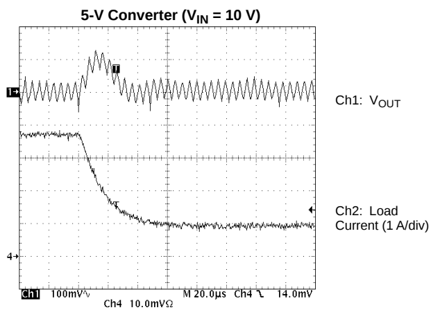
PWM Unloading
