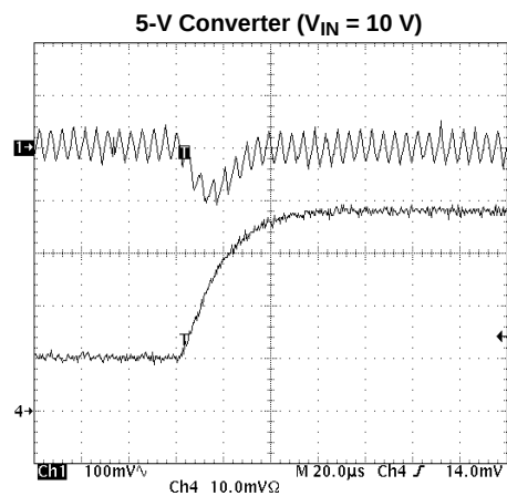
PWM Loading
