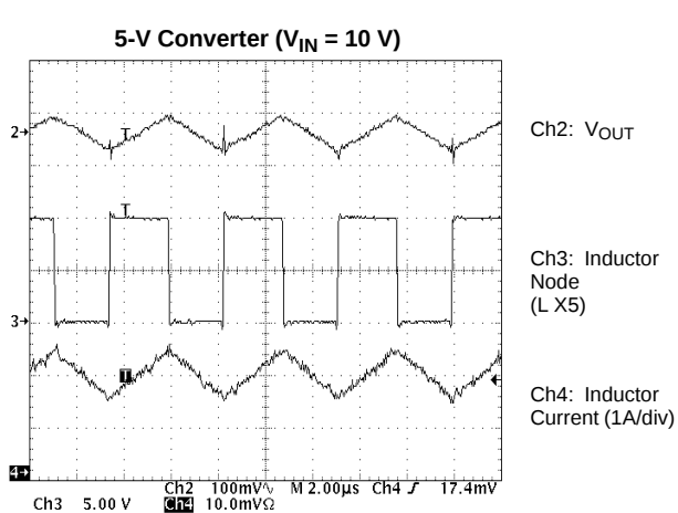
PWM Operation
