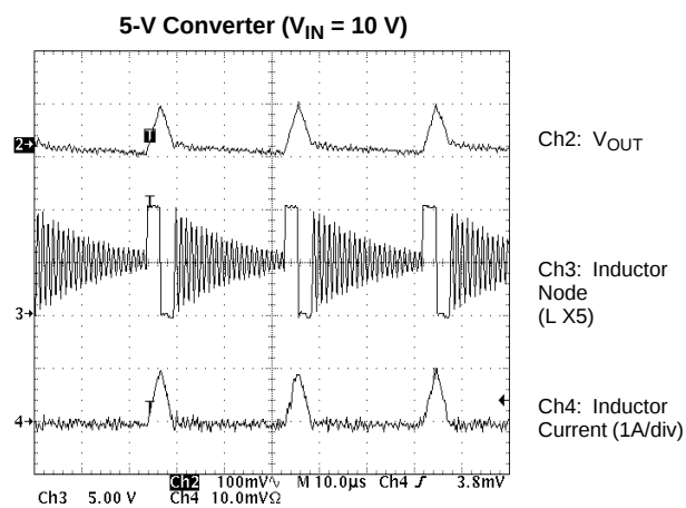
PSM Operation
