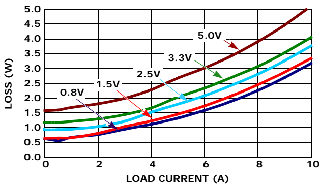
FIGURE 31. POWER LOSS vs LOAD CURRENT (12V IN )
