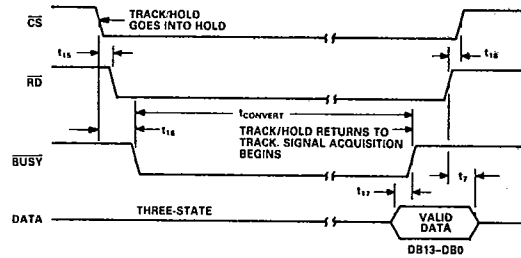
Figure 11. Mode 2 Timing Diagram, 14-Bit Parallel Read
