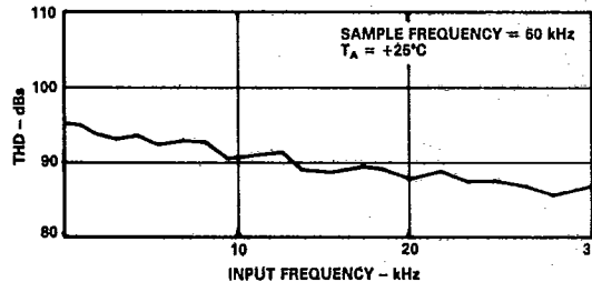
Figure 15. Total Harmonic Distortion vs. Frequency
