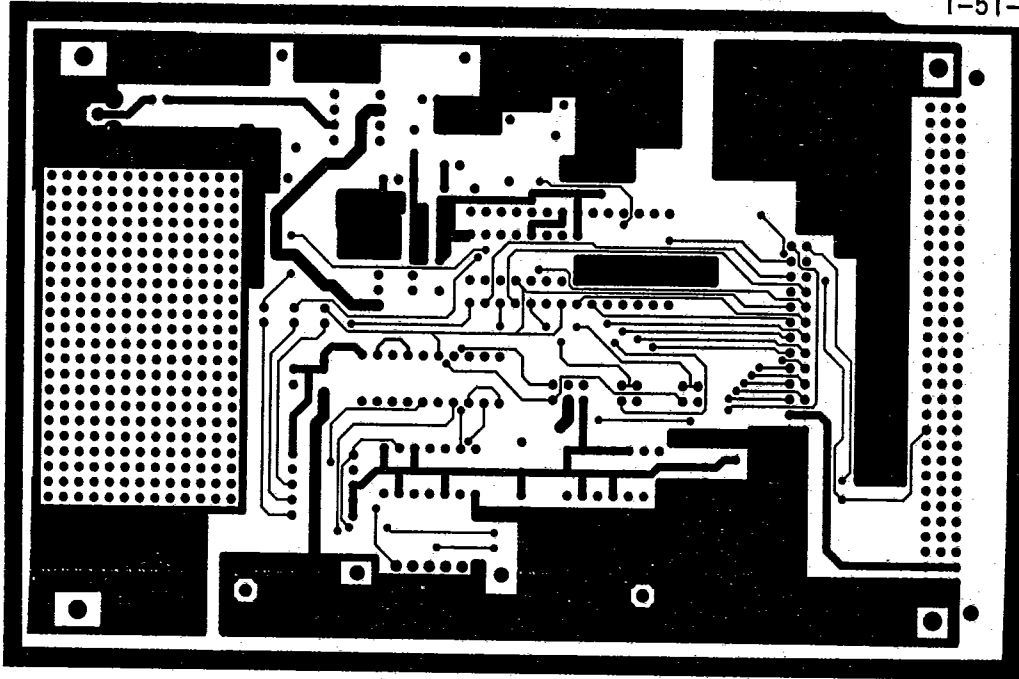
Figure 26. PCB Component Side Layout for Figure 24
