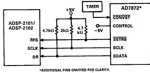
Figure 21. AD7872 to ADSP-2101/ADSP-2102 Serial Interface
