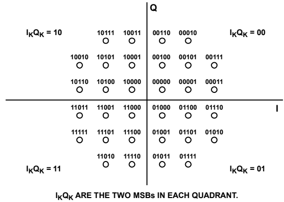
Figure 123. DVB 32-QAM Constellation
