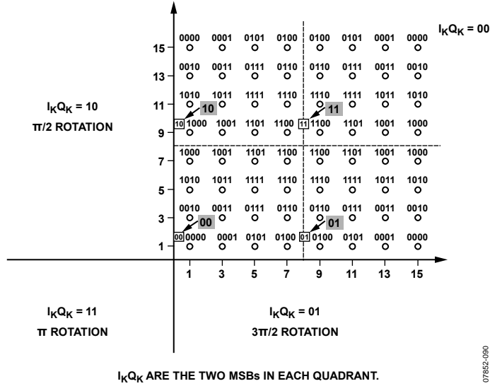
Figure 125. DVB 256-QAM Constellation
