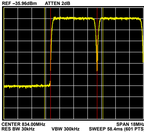
Figure 46. 4-Channel QAM ACLR, f_{OUT} = 840 MHz, Temperature = 25°C, Sum Scale = 20, Full-Scale Current = 25 mA, Span = 18 MHz, Channel 1
