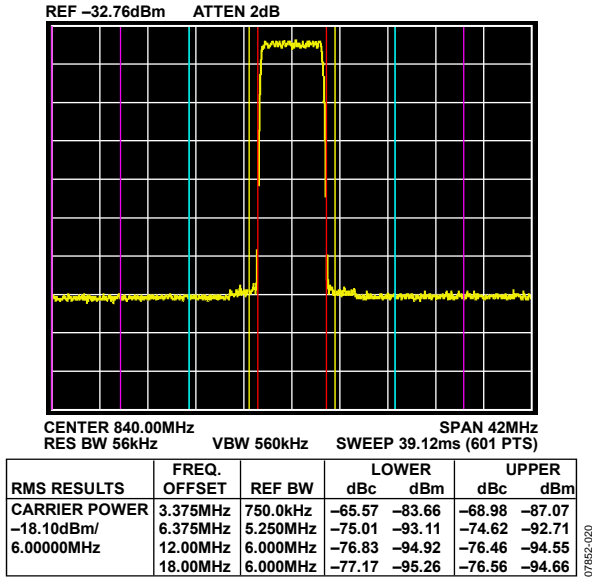
Figure 38. 1-Channel QAM ACLR, f_{OUT} = 840 MHz, Temperature = 25°C, Sum Scale = 48, Full-Scale Current = 20 mA, Span = 42 MHz
