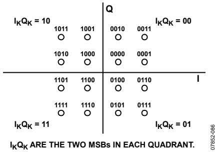
Figure 121. DVB 16-QAM Constellation
