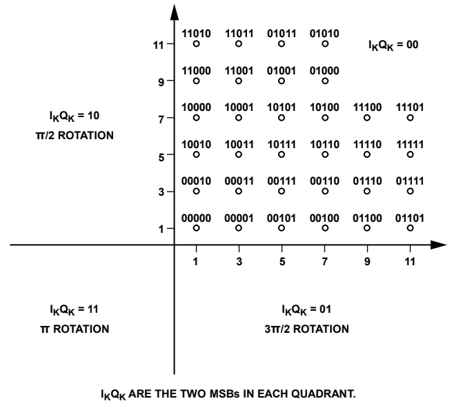
Figure 124. DVB 128-QAM Constellation
