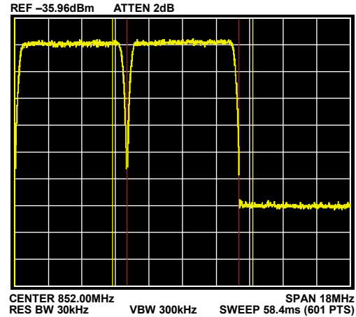
Figure 49. 4-Channel QAM ACLR, f_{OUT} = 840 MHz, Temperature = 25°C, Sum Scale = 20, Full-Scale Current = 25 mA, Span = 18 MHz, Channel 4
