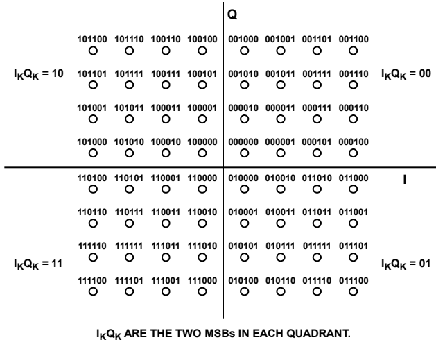
Figure 122. DVB 64-QAM Constellation
