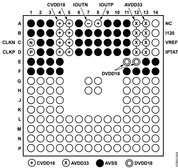
Figure 4. Clock and Analog Pins (Top View)
