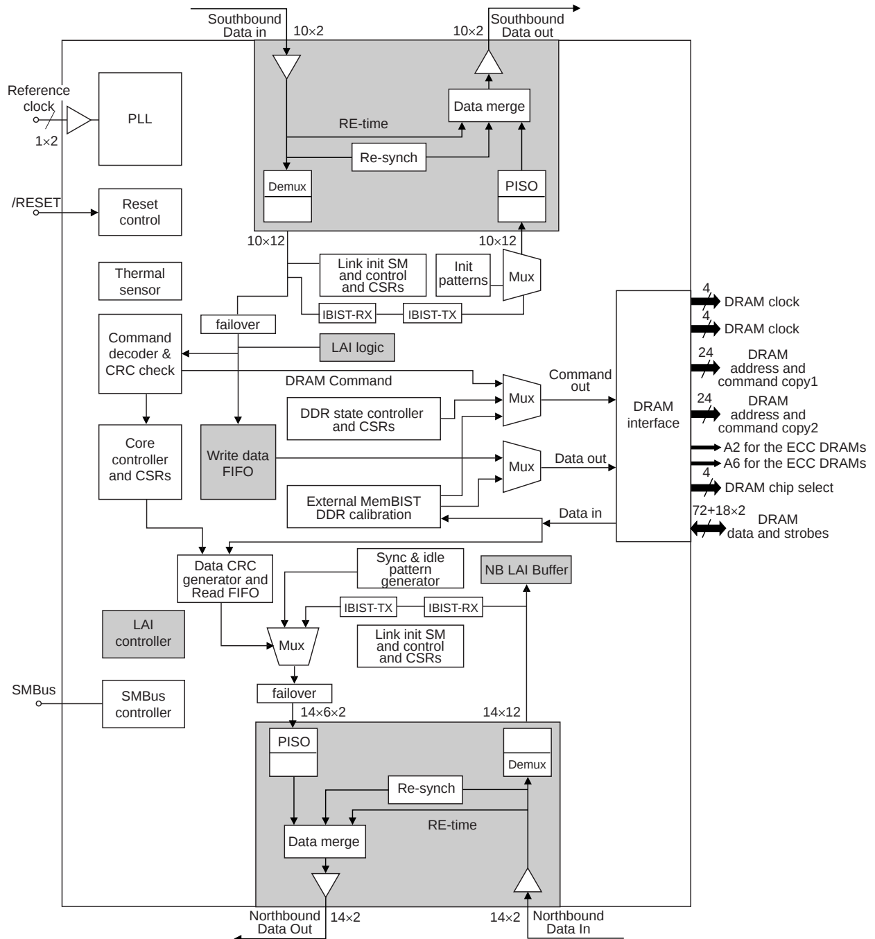
Advanced Memory Buffer Block Diagram
