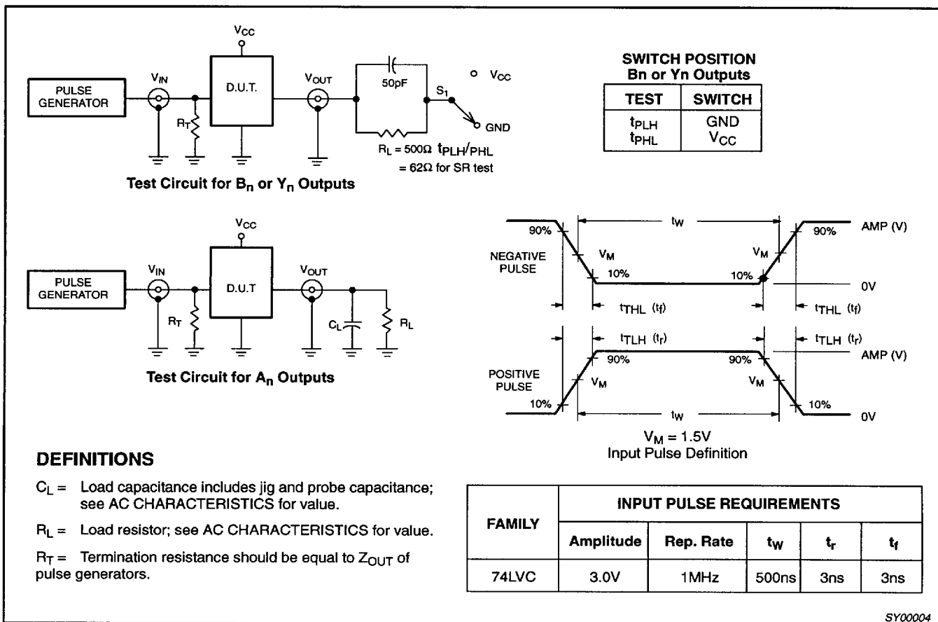
Waveform 5.
