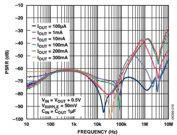
Figure 16. Power Supply Rejection Ratio vs. Frequency, V_{OUT} = 3.3\text{ V} , V_{IN} = 3.8\text{ V}
