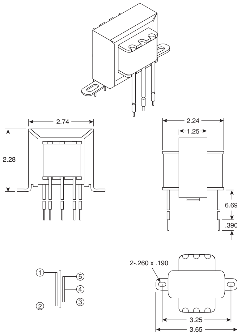
Dimensions: In.
