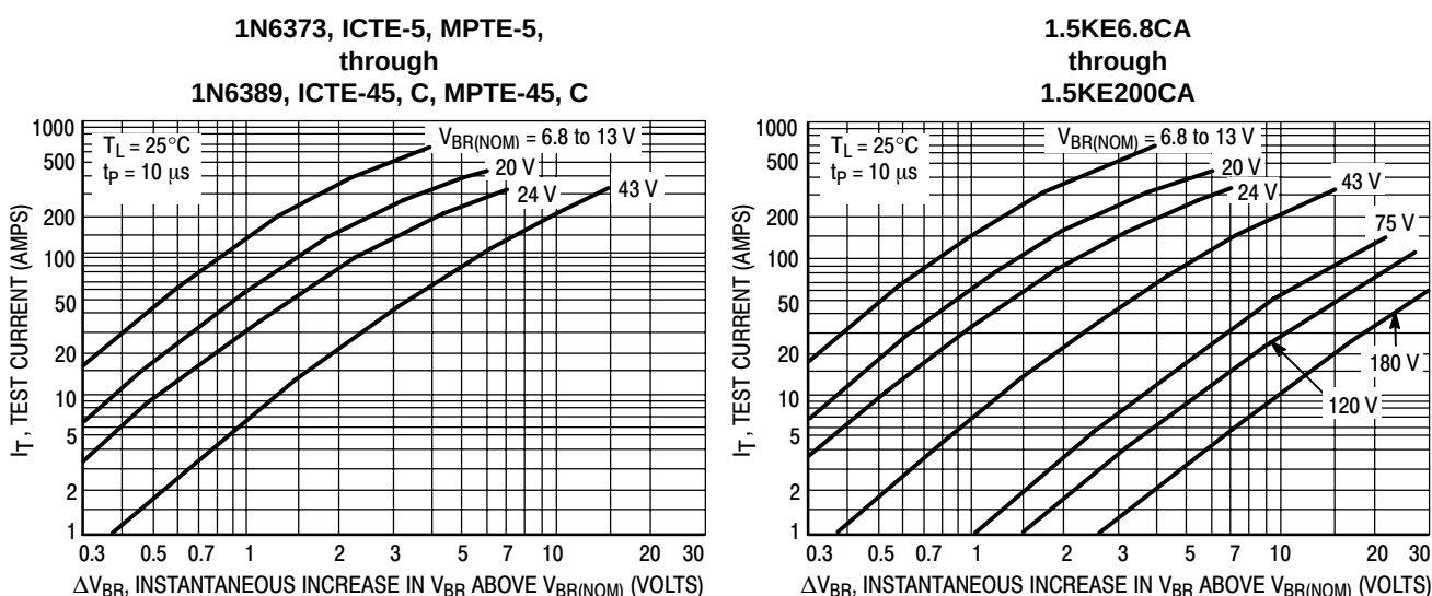
Figure 6. Dynamic Impedance
