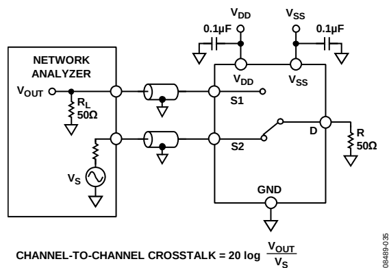
Figure 35. Channel-to-Channel Crosstalk
