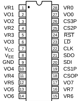
28 Pin PDIP (0.300") NN28
