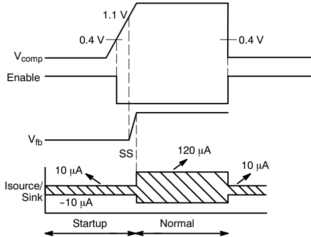
Figure 13. Soft-Start Implementation
