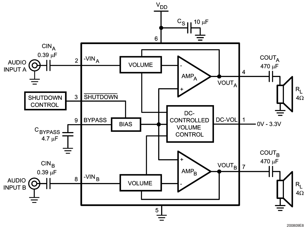
FIGURE 1. Typical LM4952 SE Audio Amplifier Application Circuit
