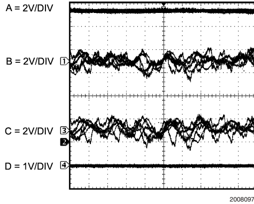
FIGURE 10. Same conditions and waveforms as shown in Figure 8, except that a 4700\mu\text{F} capacitor has been connected between the V_{\text{DD}} pin and GND (Trace A)
