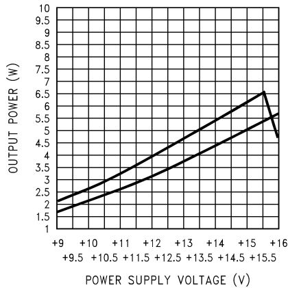
Output Power vs Power Supply Voltage
