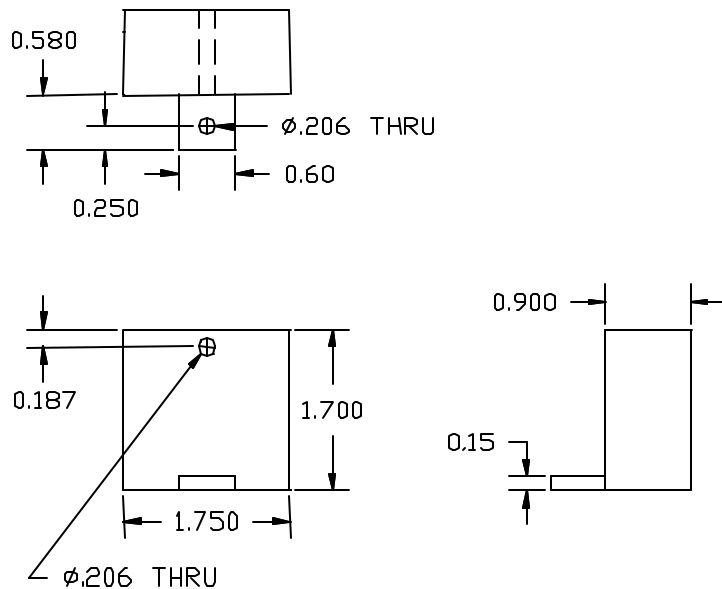
C Package
