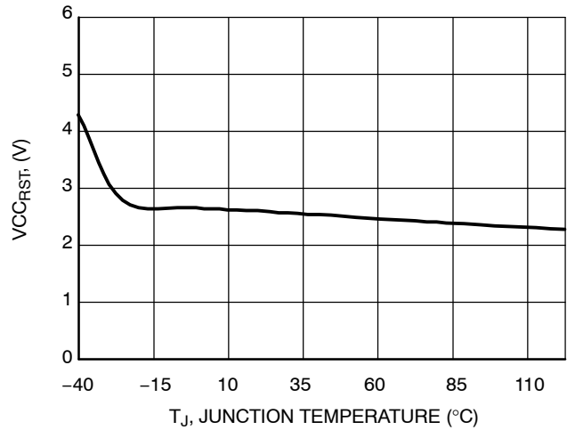
Figure 14. V_{CC} Level Below Which the Logic Resets vs. Temperature
