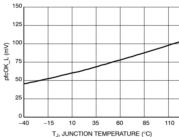
Figure 30. pfcOK Pin Low Level Voltage vs. Temperature
