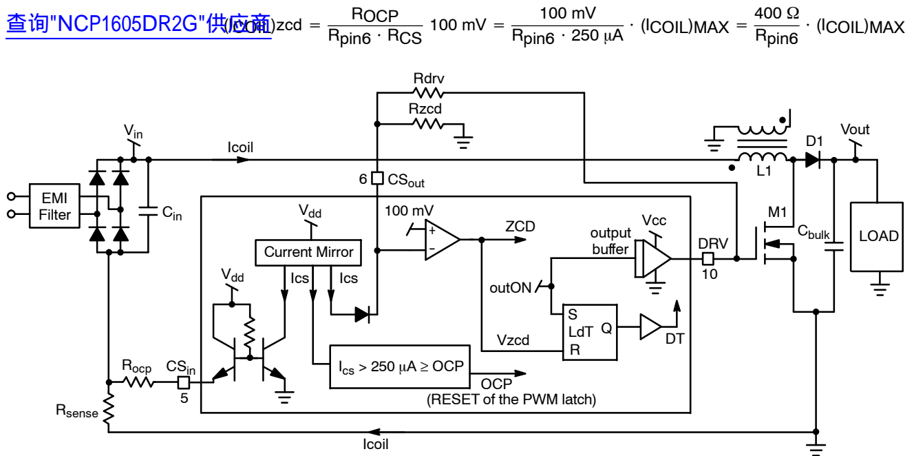
Figure 60. Current Sense Block
