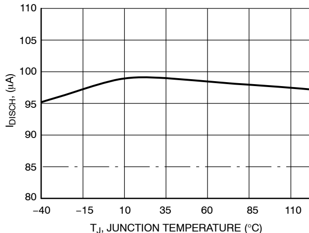
Figure 28. Oscillator Discharge Current vs. Temperature
