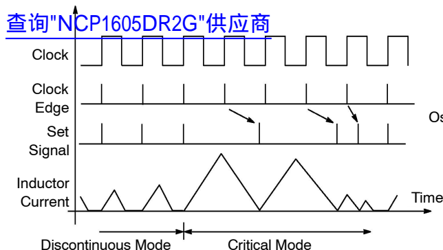
Figure 65. Oscillator Timing Diagram
