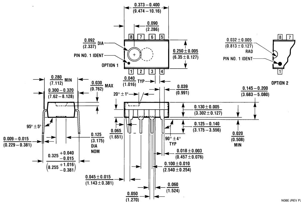
Molded Dual-In-Line Package (N) Order Number LM1881N (0°C to +70°C) NS Package Number N08E
