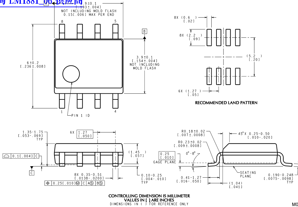
Molded Small Outline Package (M) Order Number LM1881M (0°C to +70°C) NS Package Number M08A
