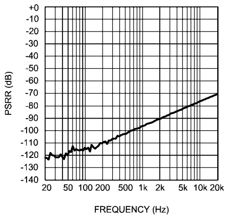
PSRR+ vs Frequency V_{CC} = 15V , V_{EE} = -2.5V R_L = 10k\Omega , V_{RIPPLE} = 200mV_{pp}
