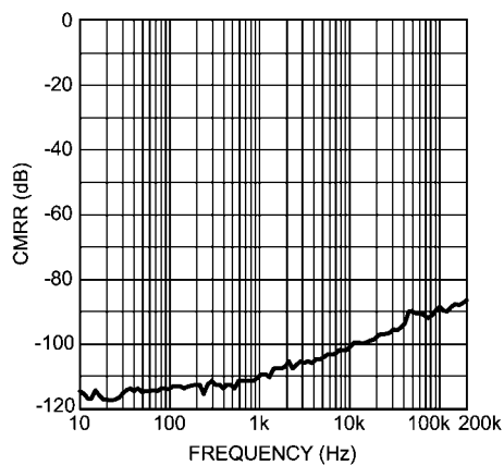
查询"LM4562_07"供应商 CMRR vs Frequency V_{CC} = 15V , V_{EE} = -17V R_L = 10k\Omega
