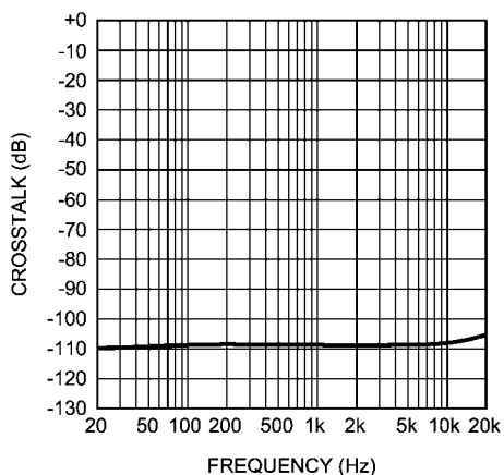
查询"LM4562"的引脚 Crosstalk vs Frequency V_{CC} = 15V, V_{EE} = -15V, V_{OUT} = 3V_{RMS} A_V = 0dB, R_L = 600\Omega
