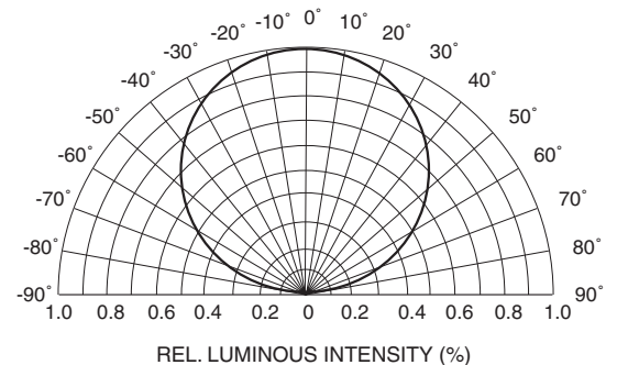
Fig. 4 Radiation Diagram
