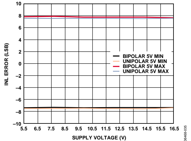
Figure 15. AD5754 Integral Nonlinearity Error vs. Supply Voltage
