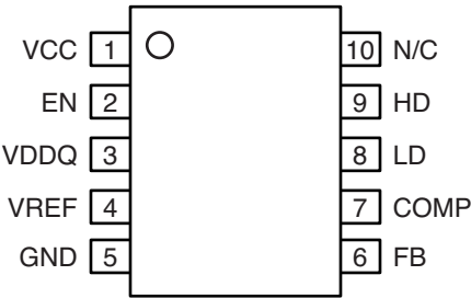
10-Lead MSOP
