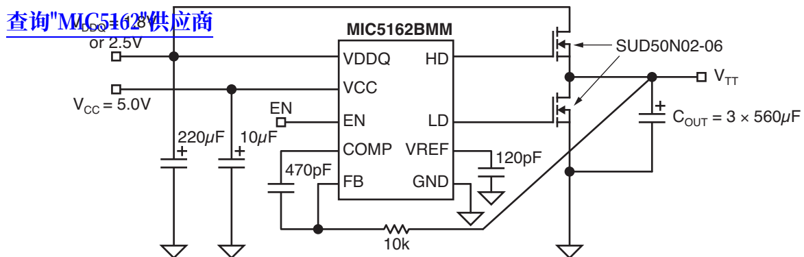
Figure 1. Test Circuit
