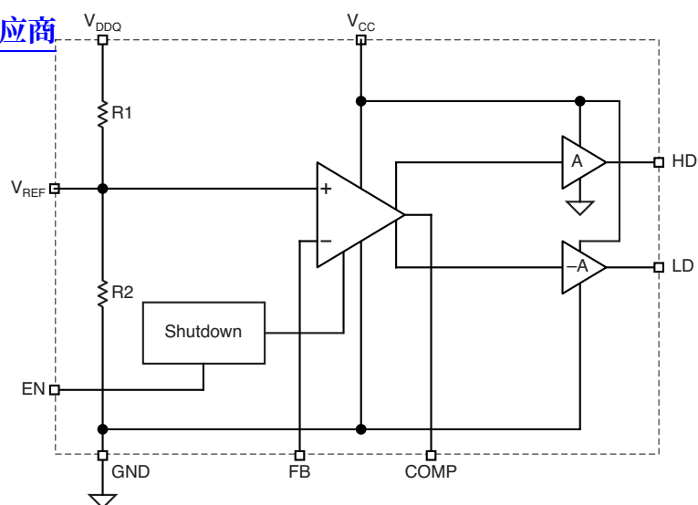
Block Diagram
