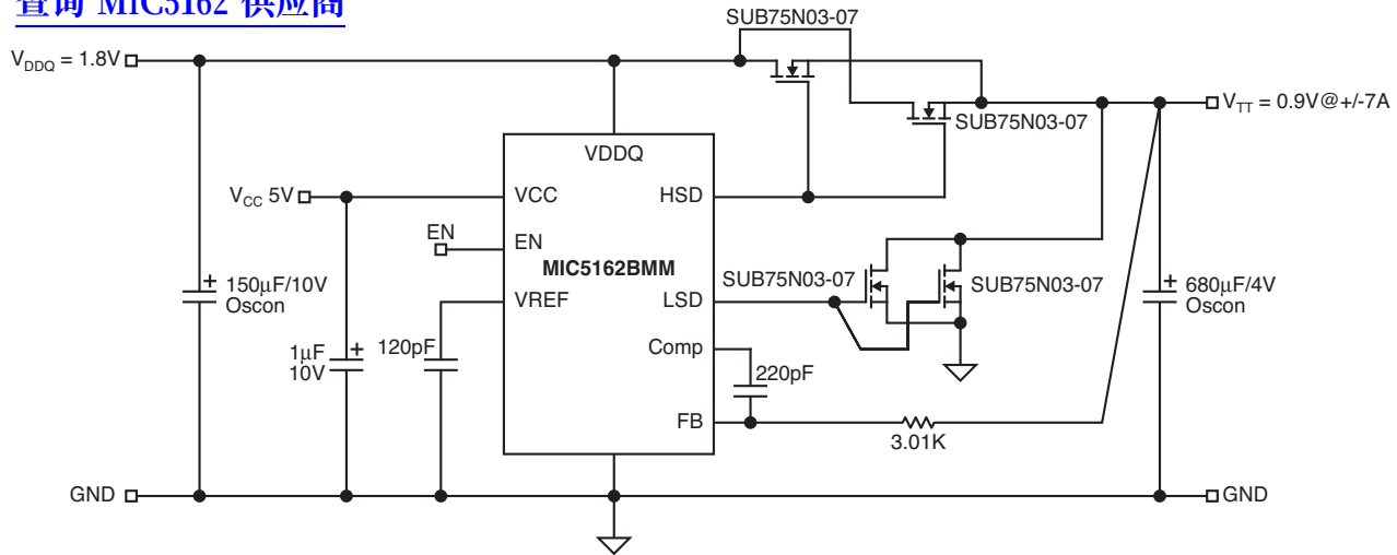
Figure 4. DDR2 Termination
