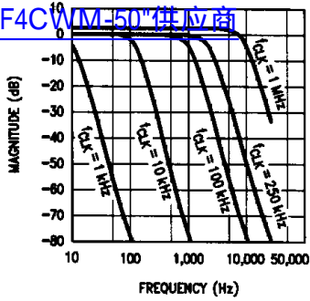
FIGURE 5a. MF4-100 Amplitude Response with ±5V Supplies
