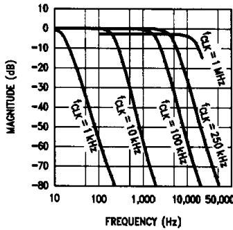
FIGURE 5d. MF4-50 Amplitude Response with ±2.5V Supplies
