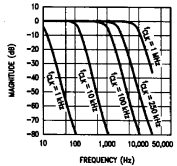
FIGURE 5c. MF4-100 Amplitude Response with ±2.5V Supplies
