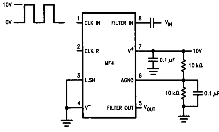
FIGURE 3. Single Supply Operation. ANGD Resistor Biased to V + / 2
