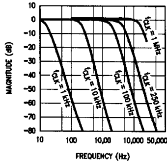
FIGURE 5b. MF4-50 Amplitude Response with ±5V Supplies
