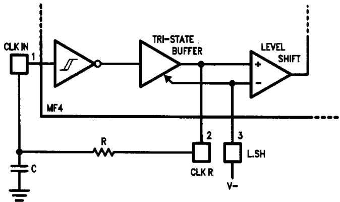
FIGURE 1. Schmitt Trigger R/C Oscillator
