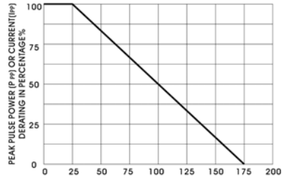
FIGURE 2 DERATING CURVE
