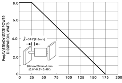
FIG. 5-STEADY STATE POWER DERATING CURVE
