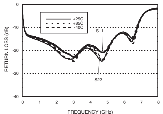
Return Loss vs. Temperature, Vfctl @ 7V [1]
