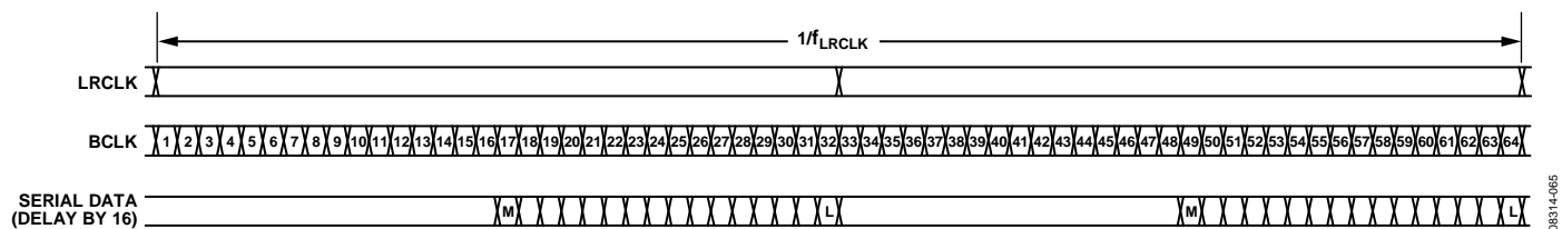
Figure 69. Serial Audio Data Delay by 16 Example
