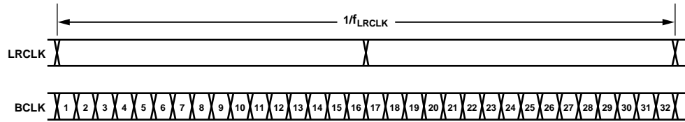
Figure 63. Example: 32 BCLK Cycles per Frame
