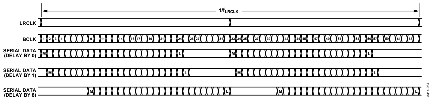
Figure 68. Serial Audio Data Delay Example Settings
